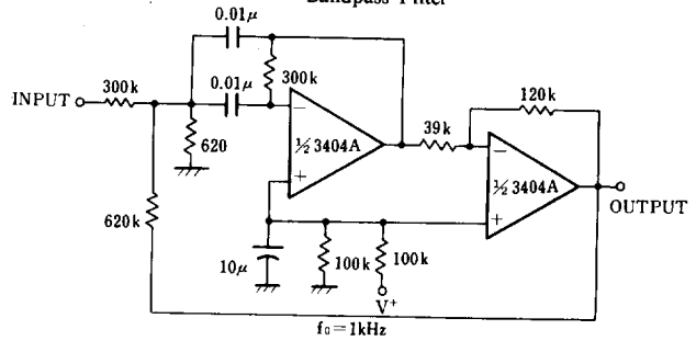
Bandpass Filter
